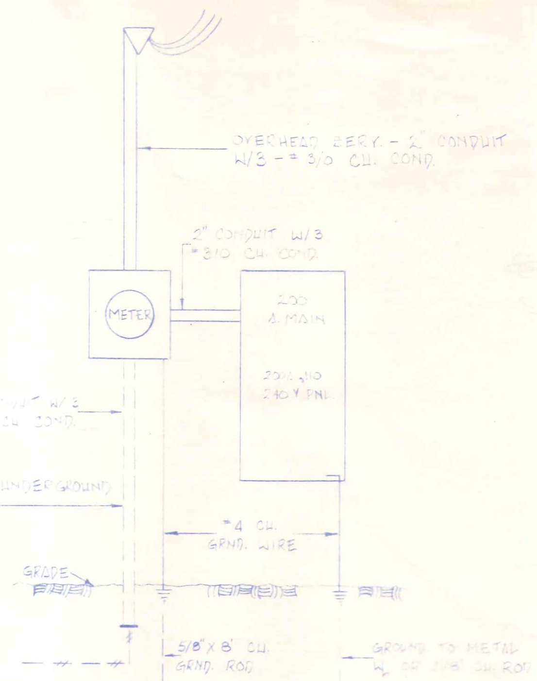
ELECTRICAL RISER DIAGRAM NO SCALE
